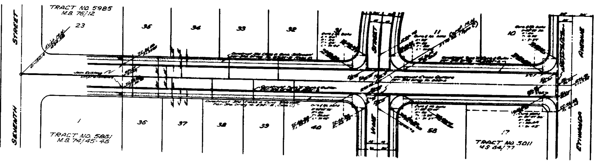
PLAN OF BURNLEY STREET See Sheet 3 for Typical Section
